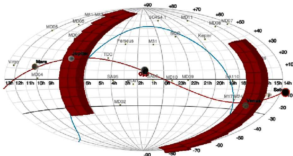
Figure 4: NEOKepler survey pattern. The highlighted red squares show all of the fields acquired in one lunation of the survey.
