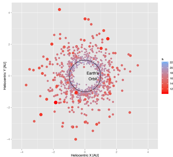
Figure 5: Positions of Kepler NEOs at time of discovery. The circle colors and sizes depict the NEO magnitudes.
